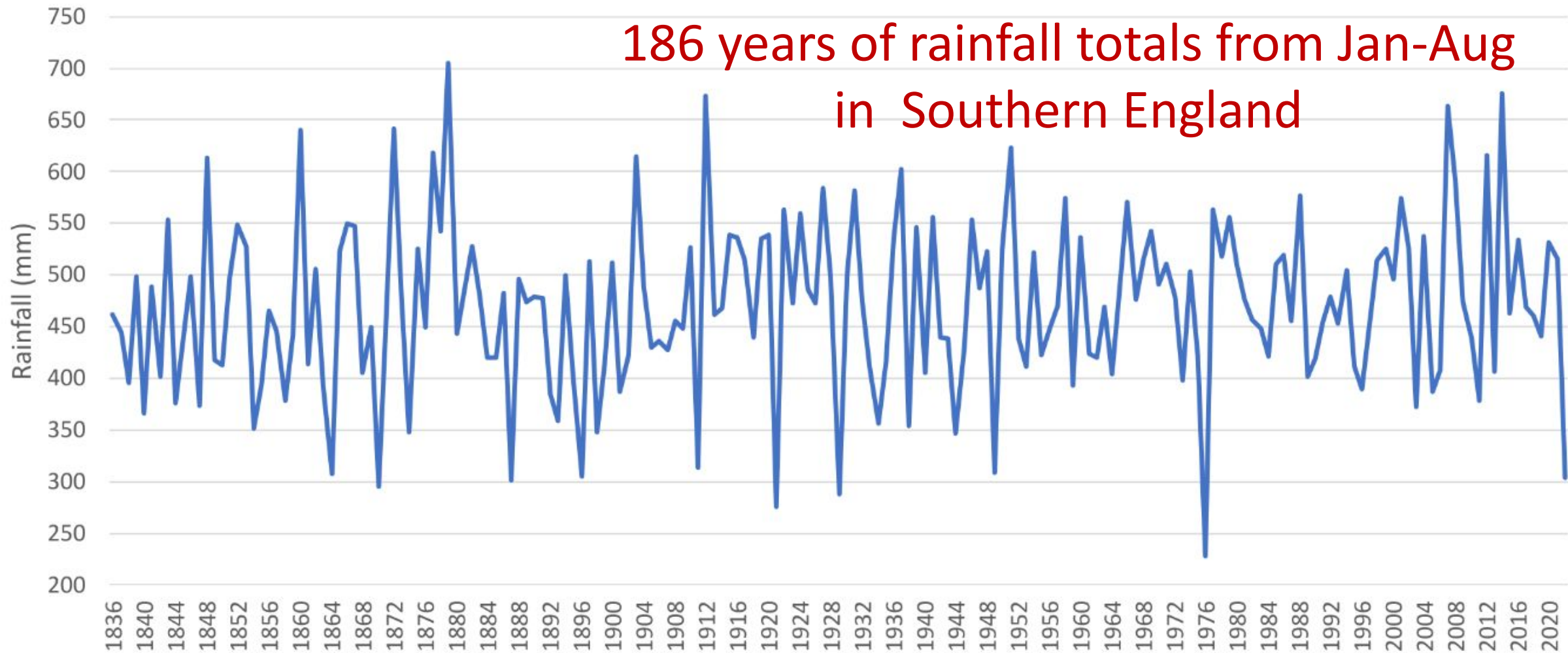
FIGURE 78 Southern England rainfall totals January–August 1836–2022.
