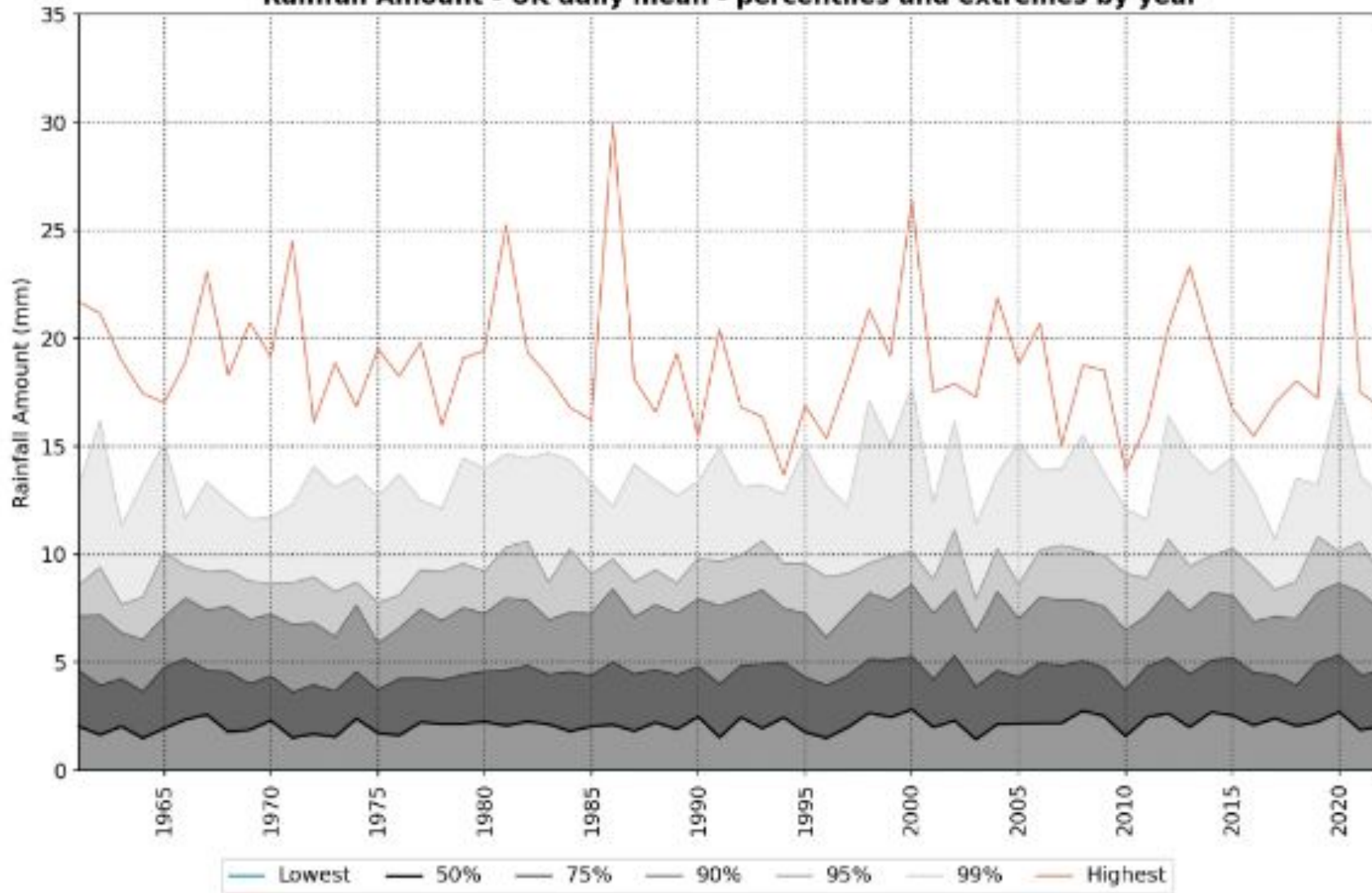
Rainfall Amount - UK daily mean - percentiles and extremes by year
